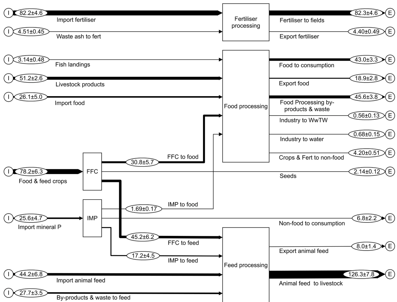
Fig. 4. Phosphorus Substance Flow diagram of the UK Food, Feed and Fertiliser processing sub-process for 2018, all values are shown as Gg/a \pm standard error and have been reconciled by STAN. FFC = Food and Feed Crops, IMP = Import Mineral Phosphorus. Line thickness of the flows is proportional to the magnitude of the flow value.
