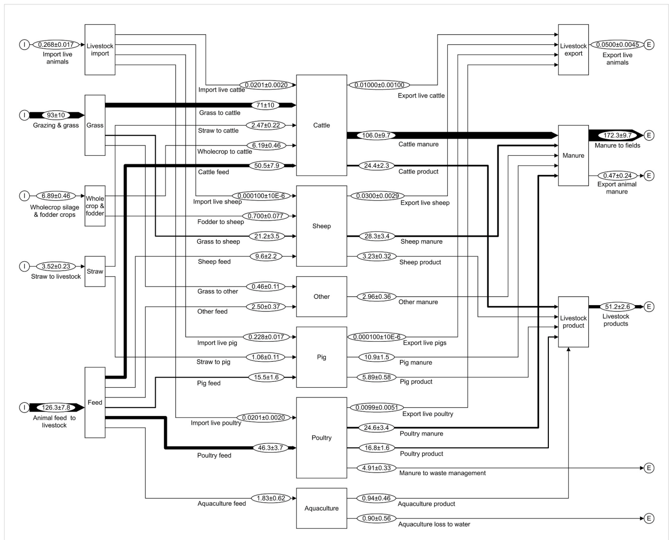
Fig. 2. Phosphorus Substance Flow diagram of the UK Animal Husbandry & Aquaculture sub-system for 2018, livestock product is as liveweight for meat animals, all values are shown as Gg/a \pm standard error and have been reconciled by STAN. Line thickness of the flows is proportional to the magnitude of the flow value.
