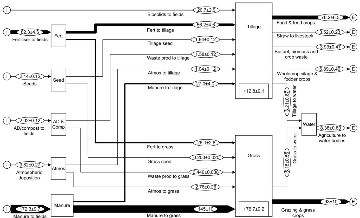
Fig. 3. Phosphorus Substance Flow diagram of the UK agricultural Crops & Grass sub-process for 2018, all values are shown as Gg/a \pm standard error and have been reconciled by STAN. Values within a process are the annual accumulation within that sector. AD = anaerobic digestion. Line thickness of the flows is proportional to the magnitude of the flow value.
